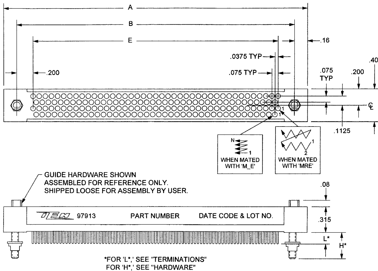
DIMENSIONS - 4 ROW [058-106]
