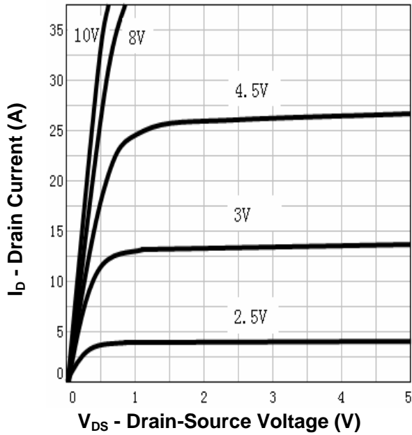
Output Characteristics
