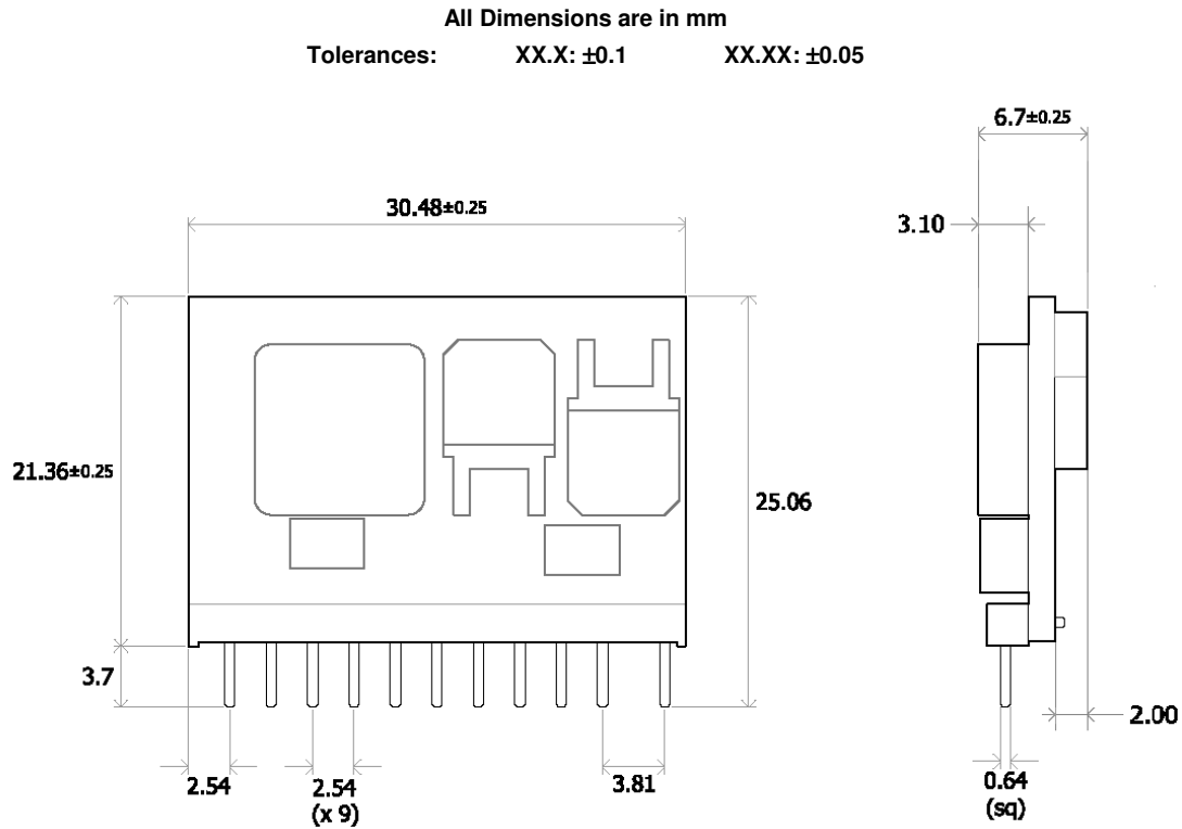
Figure 55. Mechanical Drawing
