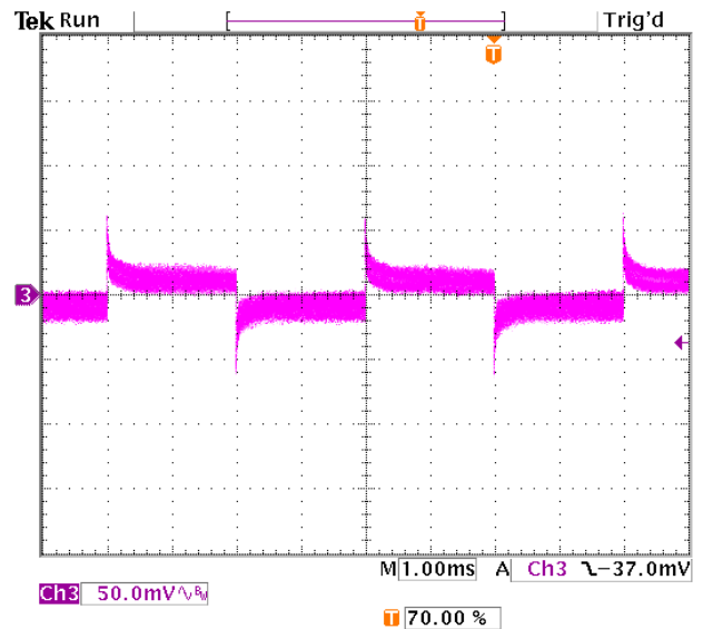
Figure 48. Transient Response with Regulation set to 3.72 mV/A
