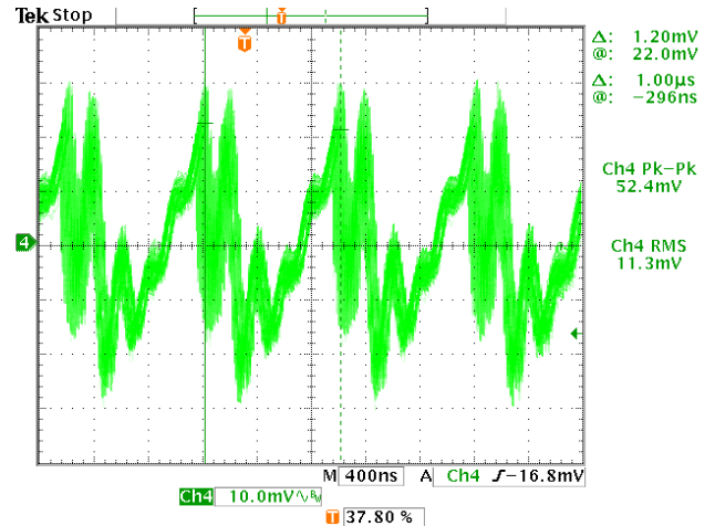
Figure 42. Input Voltage Noise, No Interleave
