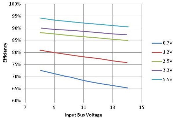
Figure 7 Efficiency vs Vin, Load=10A, Fsw=500kHz
