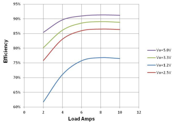
Figure 4 Efficiency vs. Load. V_{in} = 12\text{ V} , F_{sw} = 1\text{ MHz}
