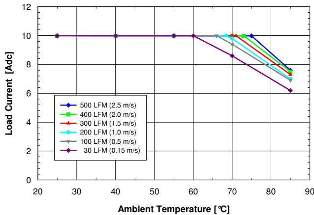
Figure 1. Available output current vs. ambient air temperature and airflow rates for converter DP8110 mounted horizontally with air flowing from input to output, MOSFET temperature \leq 120^{\circ}\text{C} , V_{in} = 12\text{ V} , V_{out} = 5\text{ V} , and F_{sw} = 500\text{ kHz}
