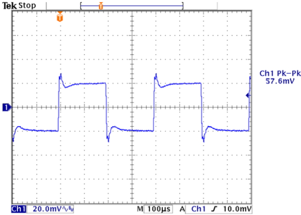
Figure 14 Transient response with non-zero Regulation.
