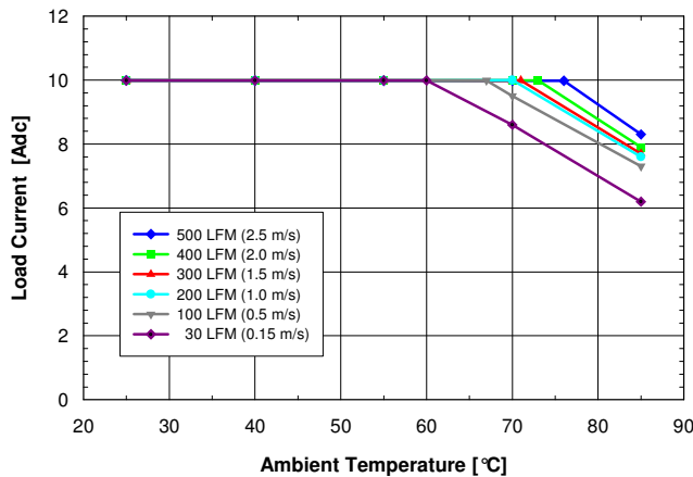
Figure 2. Available output current vs. ambient air temperature and airflow rates for converter DP8110 mounted horizontally with air flowing from input to output, MOSFET temperature \leq 120^{\circ}\text{C} , V_{in} = 12\text{ V} , V_{out} = 5\text{ V} , and F_{sw} = 1\text{ MHz}
