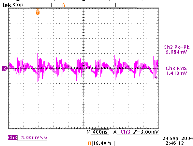
Figure 45. Output Voltage Noise, Full Load, 180° Interleave
