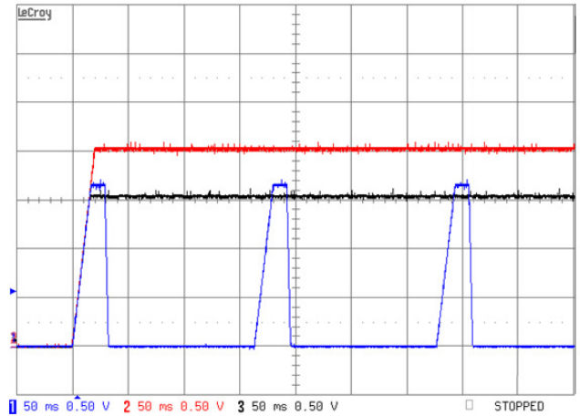
Figure 36. Turn-On into UVP on V3. The UV Fault Is Programmed To Be Non-Latching. Ch1 – Vo1, Ch2 – Vo2(Group A), Ch3 – Vo3 (Group B) Vo4 not shown.
