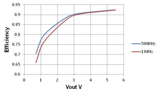
Figure 5. Efficiency vs. Output Voltage, I_{out} = 10\text{ A} , F_{sw} = 500\text{ kHz} and F_{sw} = 1\text{ MHz}
