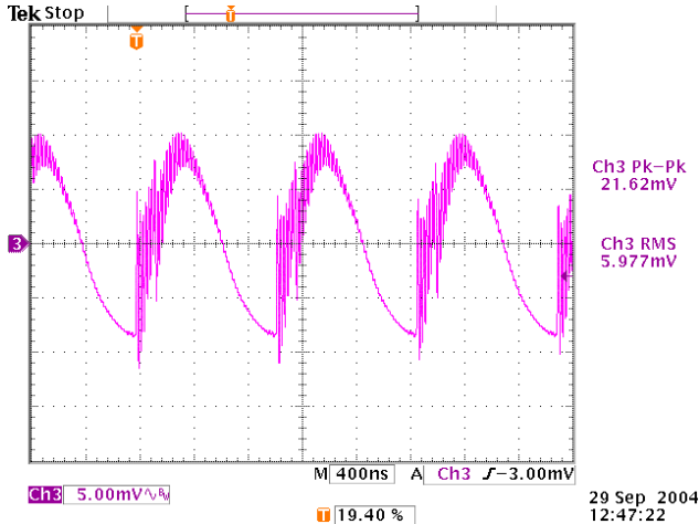
Figure 44. Output Voltage Noise, Full Load, No Interleave
