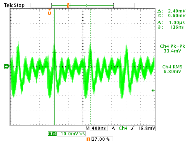
Figure 43. Input Voltage Noise with Interleave
