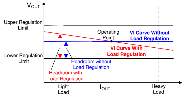
Figure 12. Optimal Voltage Positioning Concept
