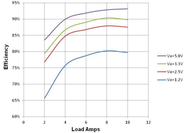
Figure 3. Efficiency vs. Load. V_{in} = 12\text{ V} , F_{sw} = 500\text{ kHz}
