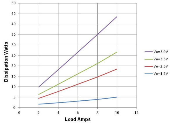
Figure 8. Dissipation vs Load, Vin=12V, Fsw=500kHz
