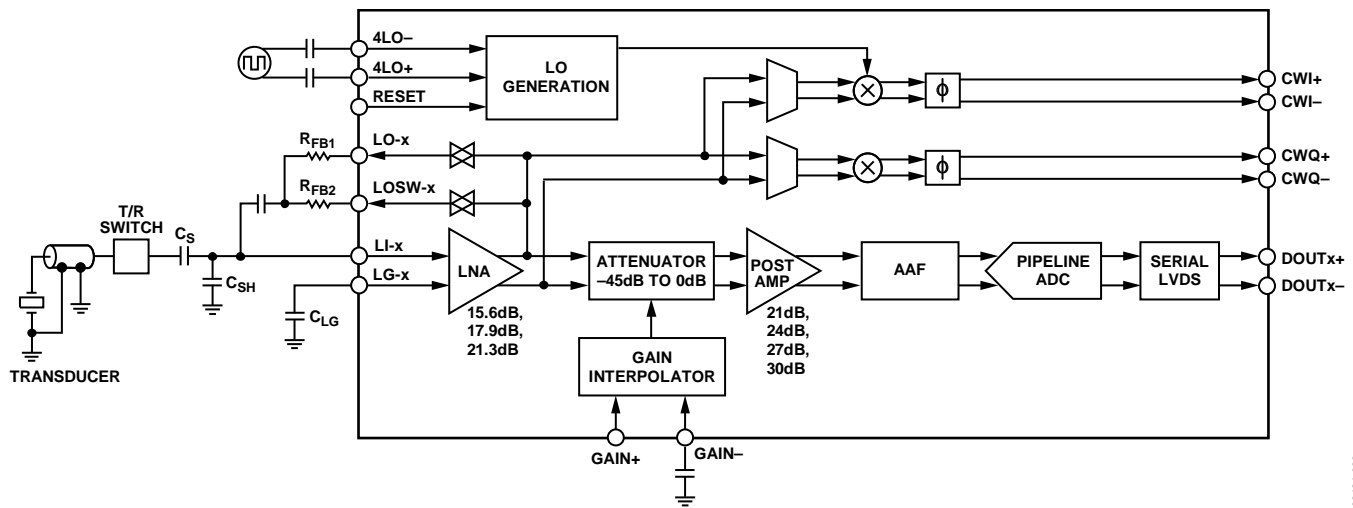
Figure 38. Simplified Block Diagram of a Single Channel
