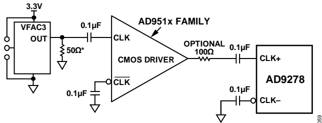
Figure 54. Single-Ended 3.3 V CMOS Sample Clock
