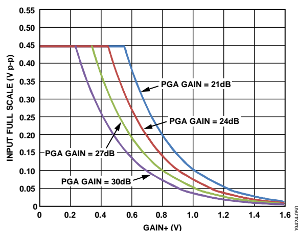
Figure 42. LNA with 21.3 dB Gain Setting/VGA Full-Scale Limitations
