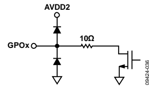
Figure 36. Equivalent GPOx Output Circuit
