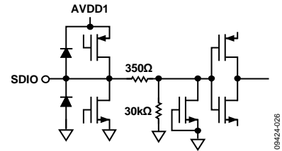
Figure 26. Equivalent SDIO Input Circuit
