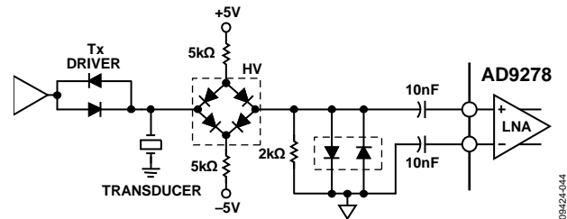
Figure 47. Input Overload Protection
