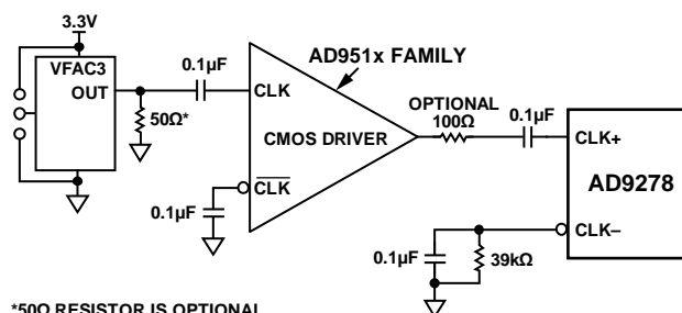
Figure 53. Single-Ended 1.8 V CMOS Sample Clock
