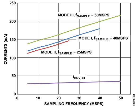
Figure 56. Supply Current vs. f_{SAMPLE} for f_{IN} = 5 MHz
