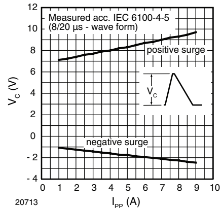
20713 Figure 6. Typical Peak Clamping Voltage vs. Peak Pulse Current I_{PP}
