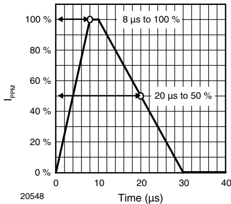
20548 Figure 2. 8/20 \mu s Peak Pulse Current Wave Form acc. IEC 61000-4-5
