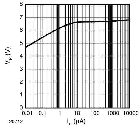
20712 Figure 5. Typical Reverse Voltage V_R vs. Reverse Current I_R
