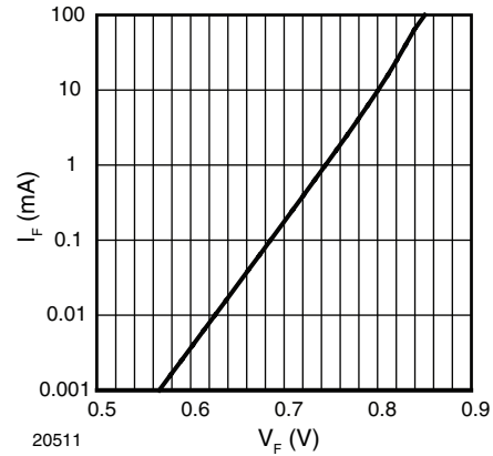
20511 Figure 4. Typical Forward Current I_F vs. Forward Voltage V_F
