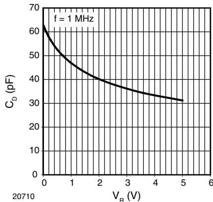
20710 Figure 3. Typical Capacitance C_D vs. Reverse Voltage V_R
