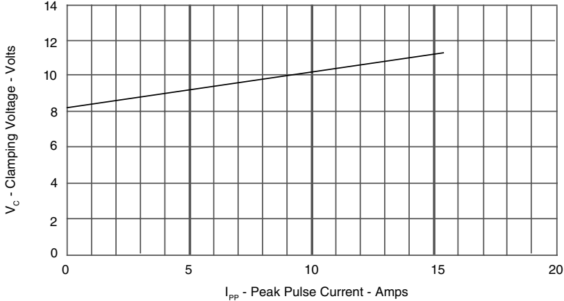
FIGURE 5 TYPICAL CLAMPING VOLTAGE VS PEAK PULSE CURRENT FOR ULC0404FC05C
