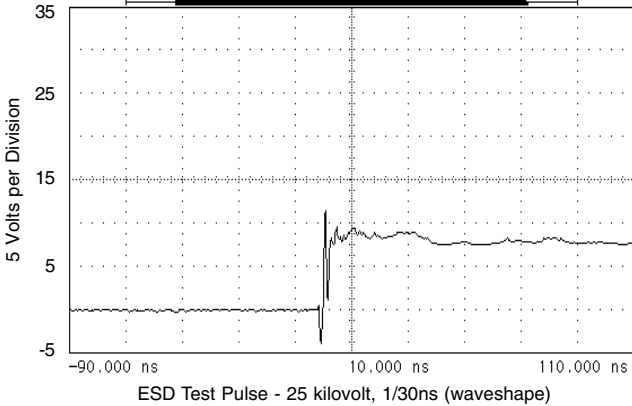
FIGURE 4 OVERSHOOT & CLAMPING VOLTAGE FOR ULC0404FC05C
