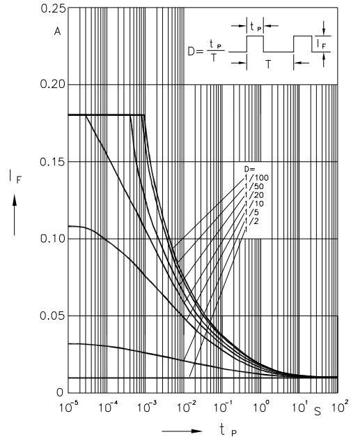
Permissible Pulse Handling Capability Duty cycle D=parameter, TA=85°C
