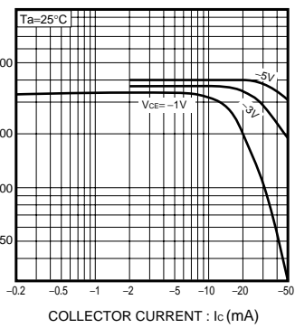
Fig.3 DC current gain vs. collector current
