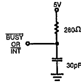
BUSY Output Load (CY7C130/CY7C131 ONLY) C132-8
