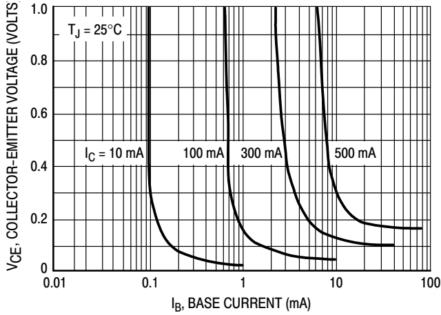
Figure 21. Saturation Region
