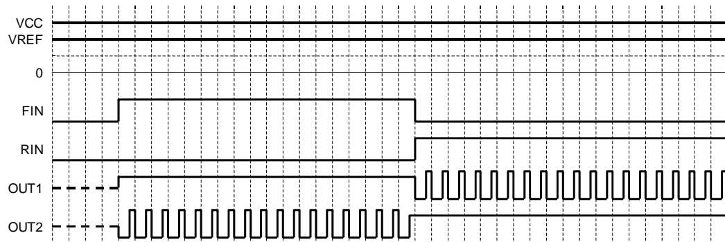
Fig.35 VREF control operation (timing chart)
