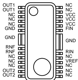
Fig.6 HSOP25 (TOP VIEW)
