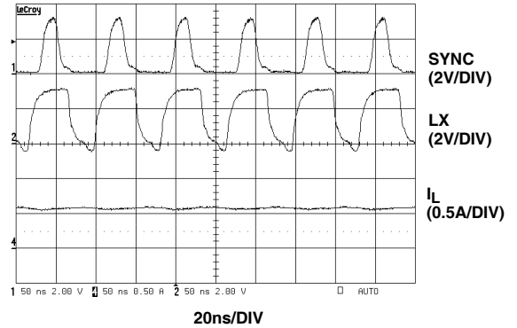
FIGURE 10. EXTERNAL SYNCHRONIZATION TO 12MHz
