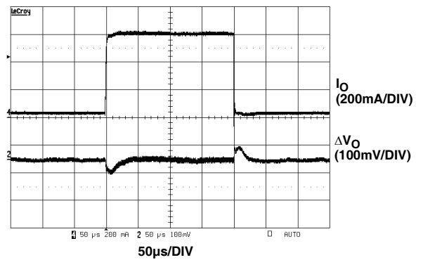
FIGURE 12. LOAD TRANSIENT RESPONSE (30mA TO 600mA)
