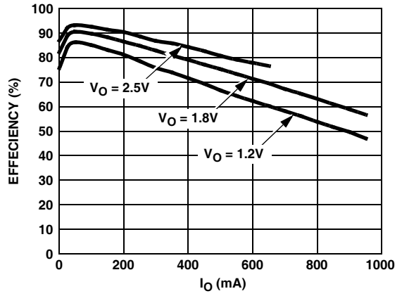
FIGURE 2. EFFICIENCY vs I_O AT 3.3V
