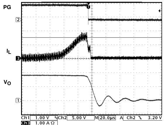
FIGURE 16. OVERCURRENT SHUTDOWN
