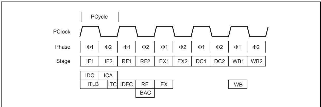
Figure 4-20. JALR Instruction Pipeline Activities (VR4181)
