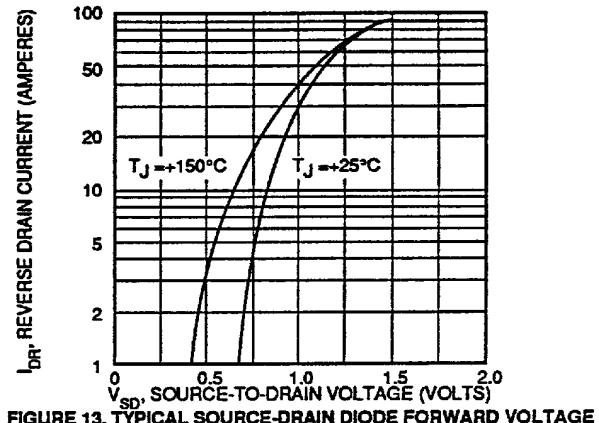
FIGURE 13, TYPICAL SOURCE-DRAIN DIODE FORWARD VOLTAGE
