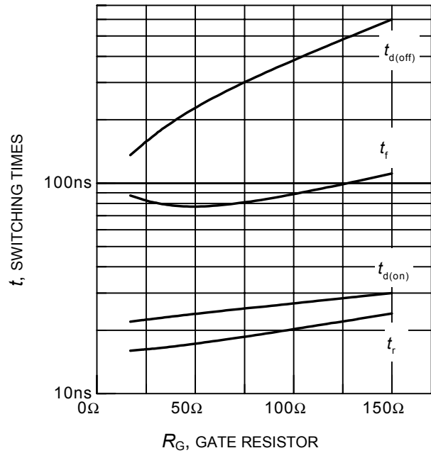
Figure 10. Typical switching times as a function of gate resistor (inductive load, T_j = 150^\circ\text{C} , V_{CE} = 400\text{V} , V_{GE} = 0/+15\text{V} , I_C = 6\text{A} , V_{GE} = 0/+15\text{V} , I_C = 6\text{A} , Dynamic test circuit in Figure E)
