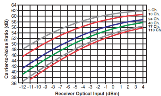
Carrier-to-Noise Performance
