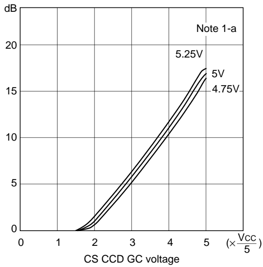
CS CCD gain control characteristics
