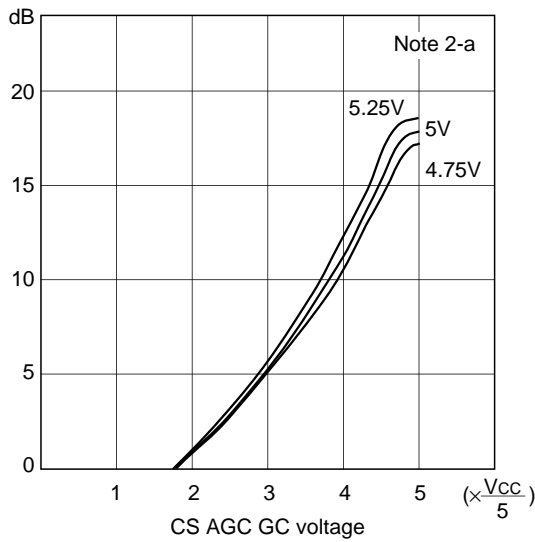
CS AGC gain control characteristics
