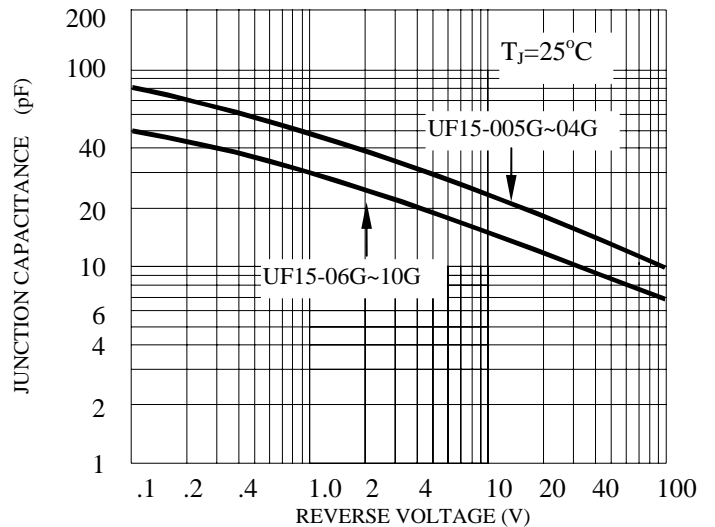
FIG. 6-TYPICAL JUNCTION CAPACITANCE
