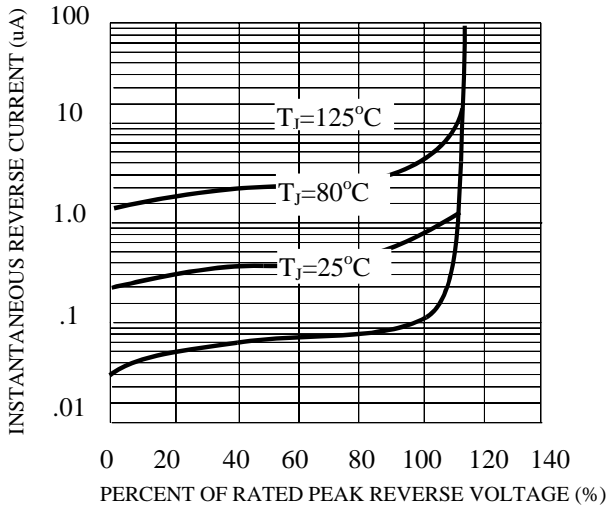
FIG. 3-TYPICAL REVERSE CHARACTERISTICS
