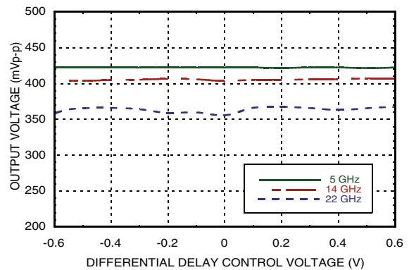
Single-Ended Output Swing vs. Delay Control Voltage [1][2][4][6]
