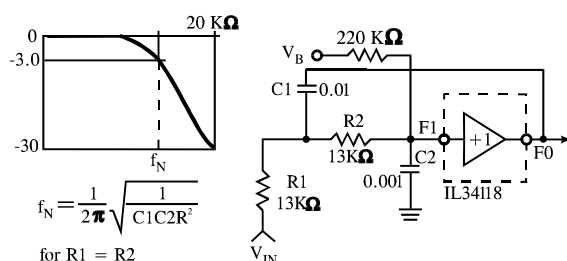
Figure 7. Low Pass Filter
