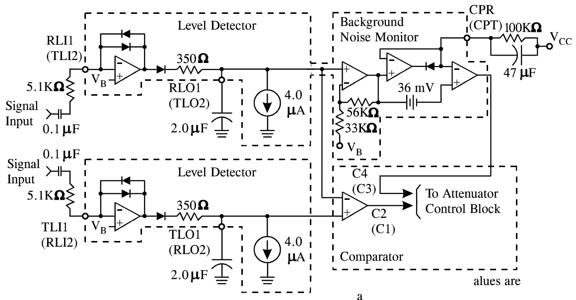
Figure 2. Level Detectors
