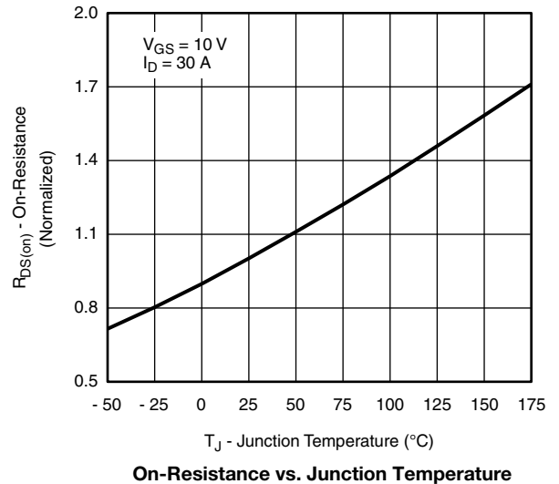
R_{DS(on)} - On-Resistance (Normalized) T_J - Junction Temperature ( ^\circ\text{C} ) V_{GS} = 10\text{ V} , I_D = 30\text{ A} On-Resistance vs. Junction Temperature
