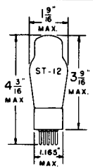
GLASS BULB SMALL 6 PIN BASE 25Z5
