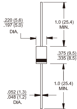
Dimensions in inches and (millimeters) Marking Diagram
