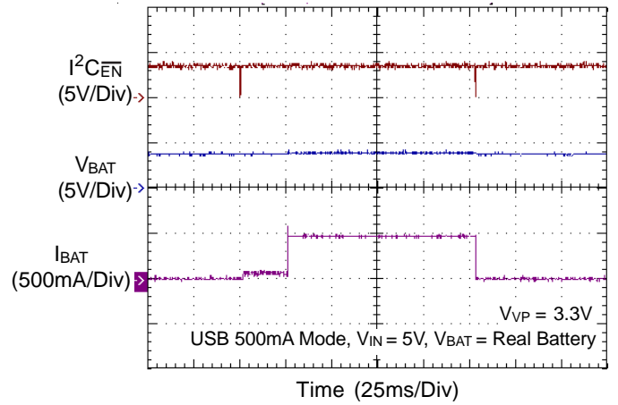
Charger On/Off Control from ENCH
