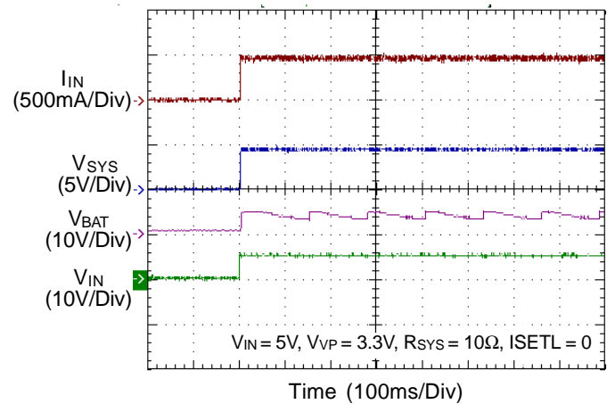
VIN Hot-Plug with NTC/without Battery
