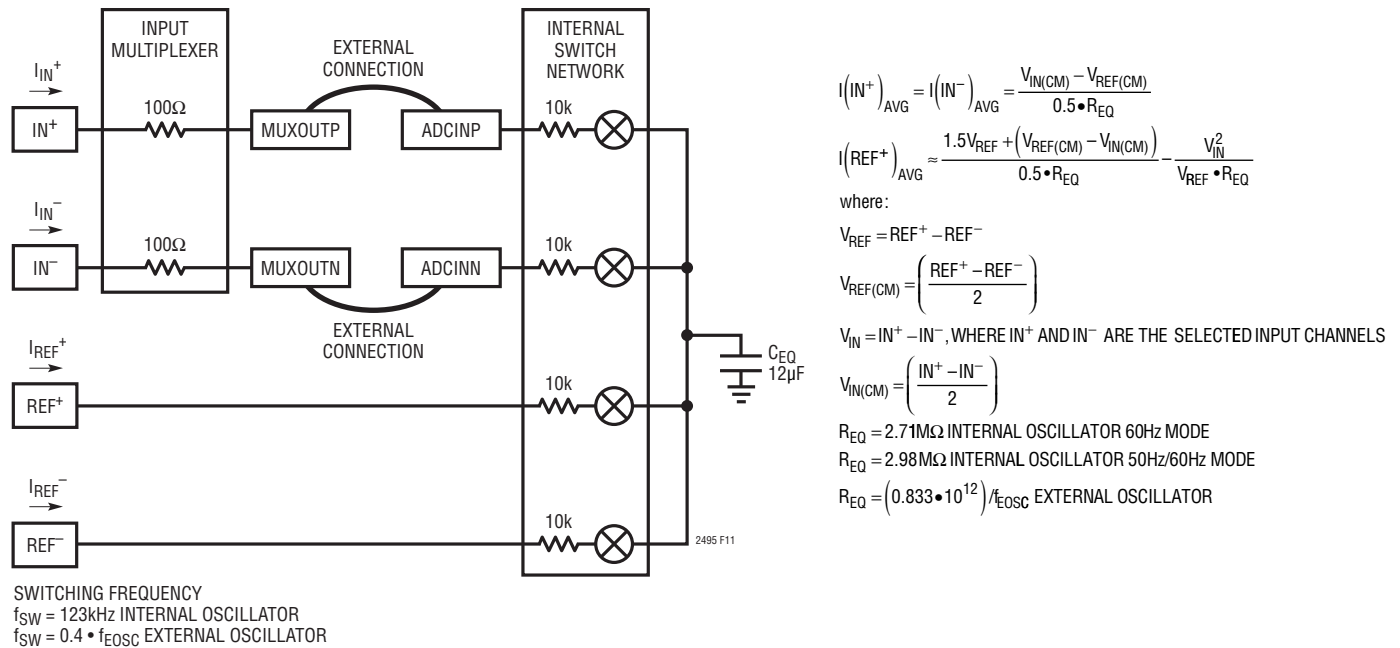
Figure 11. Equivalent Analog Input Circuit
