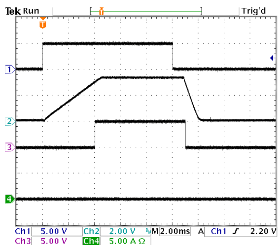
Power Up/Down at No Load: V_{IN}/V_{OUT} = 5V/3.3V , 47nF soft-start capacitor, C_{OUT} \approx 50\mu F Ch.1: ENABLE, Ch. 2: V_{OUT} , Ch. 3: POK, Ch.4: I_{OUT}
