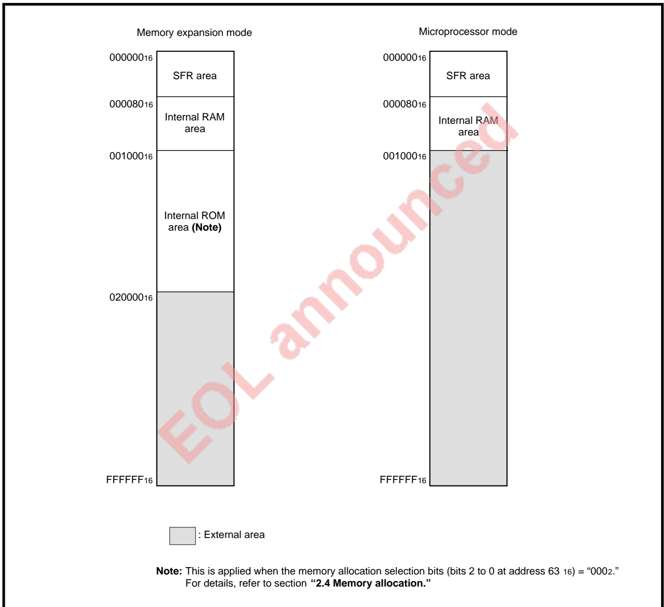
Fig. 12.1.2 External area
