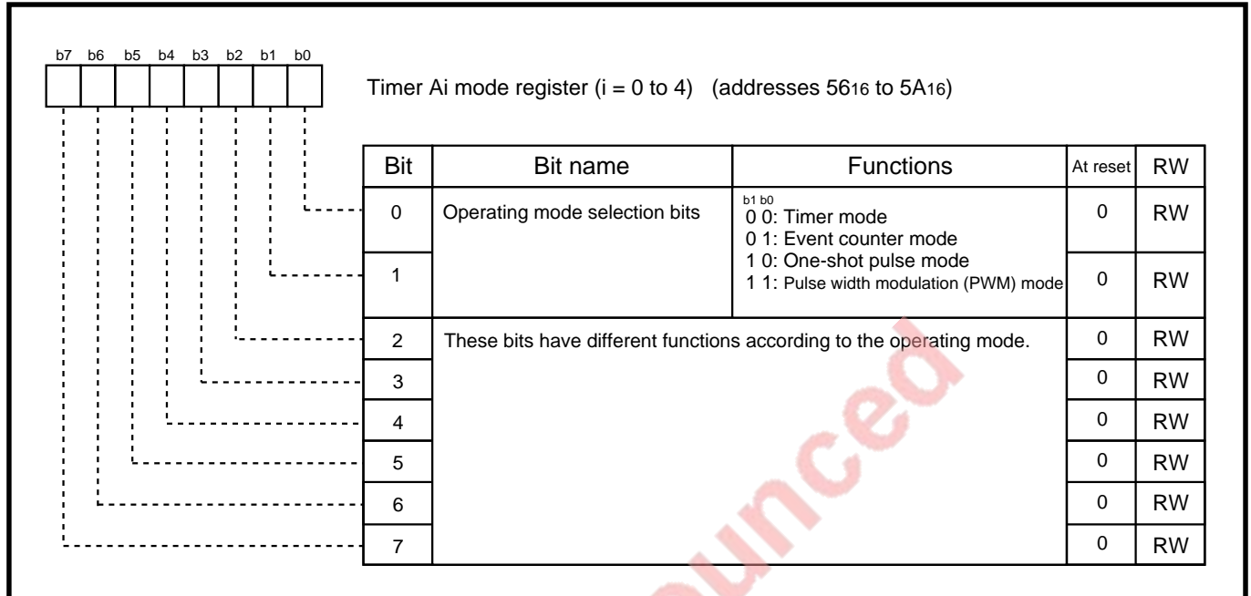
Fig. 6.2.3 Structure of timer Ai mode register
