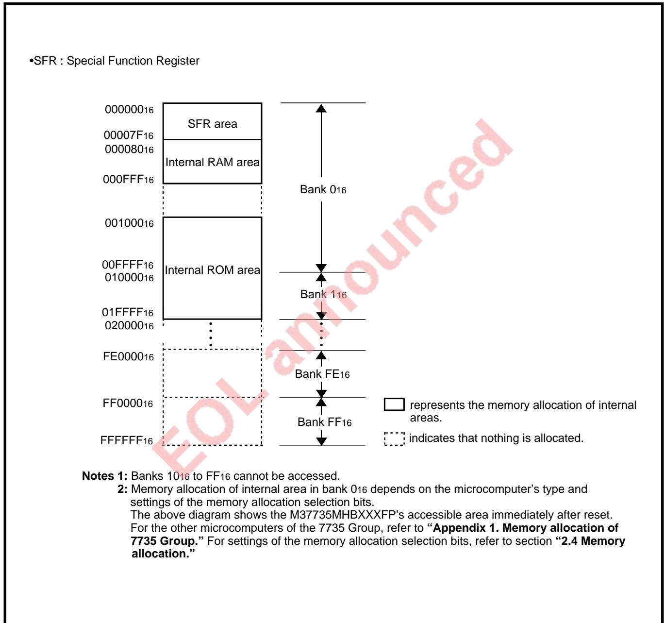
Fig. 2.3.1 M37735MHBXXFP's accessible area
