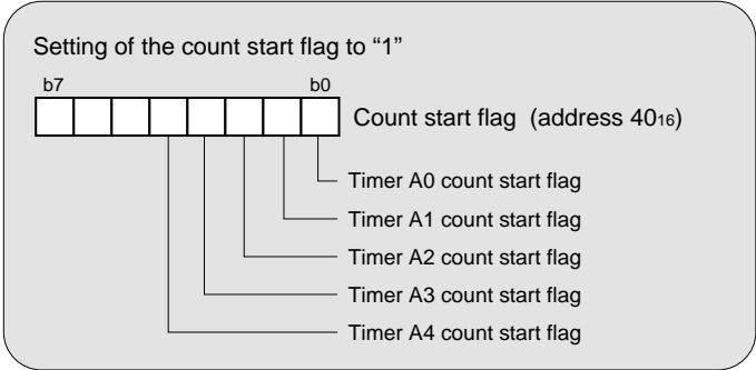
Fig. 6.4.4 Initial setting example for registers related to event counter mode (2)
