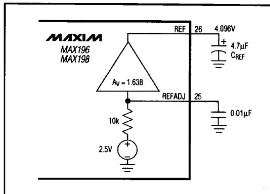
Figure 9a. Internal Reference
