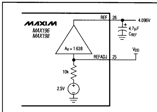
Figure 9b. External Reference, Reference at REF
