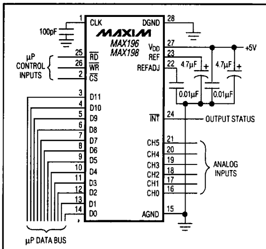
Figure 3. Operational Diagram
