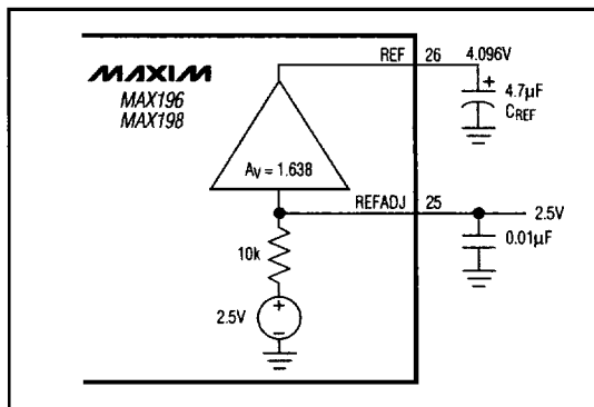
Figure 9c. The external reference overdrives the internal reference.
