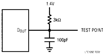
Load Circuit for t_{dD0} , t_r and t_f
