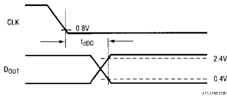
Voltage Waveform for D_{OUT} Delay Time, t_{dD0}
