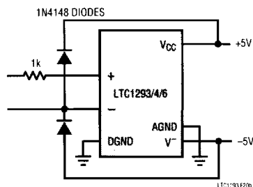
Figure 20b. Overvoltage Protection for Inputs
