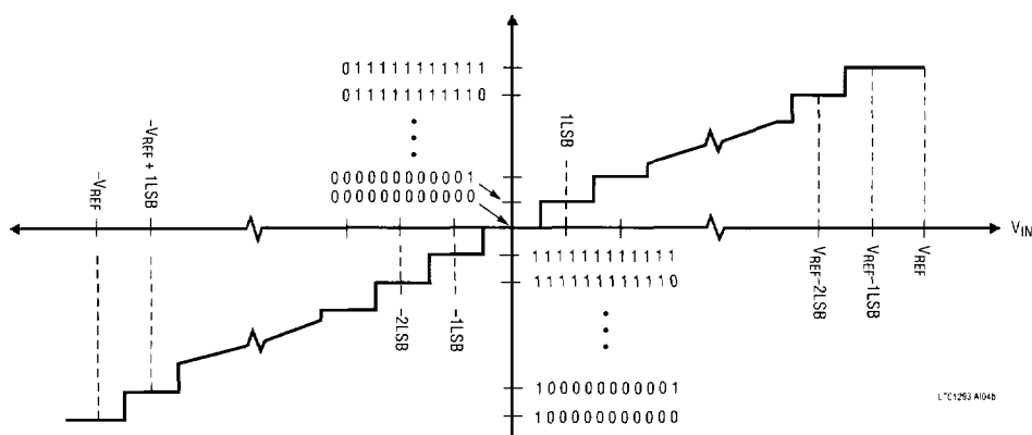
Bipolar Output Code (UNI = 0)
