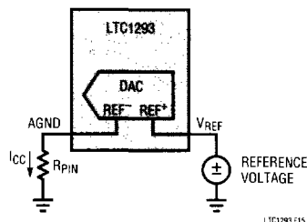
Figure 15. Parasitic Pin Resistance ( R_{PIN} )
