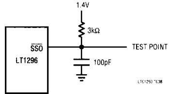
Load Circuit for t_{enSS0} and t_{disSS0}
