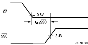
Voltage Waveform for t_{disSS0}
