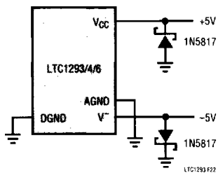
Figure 22. Power Supply Reversal
