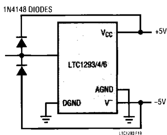
Figure 19. Overvoltage Protection for Inputs
