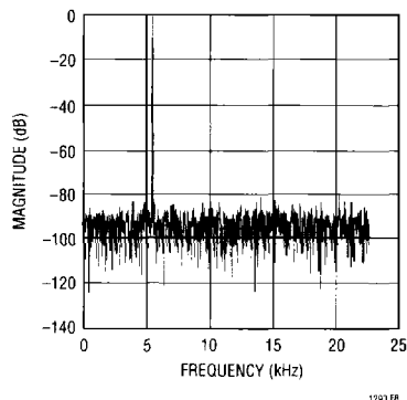
Figure 18. LTC1294 FFT Plot f_{IN1} = 5.1\text{kHz} , f_{IN2} = 5.6\text{kHz} , f_S = 45.4\text{kHz} with \pm 5\text{V} Supplies
