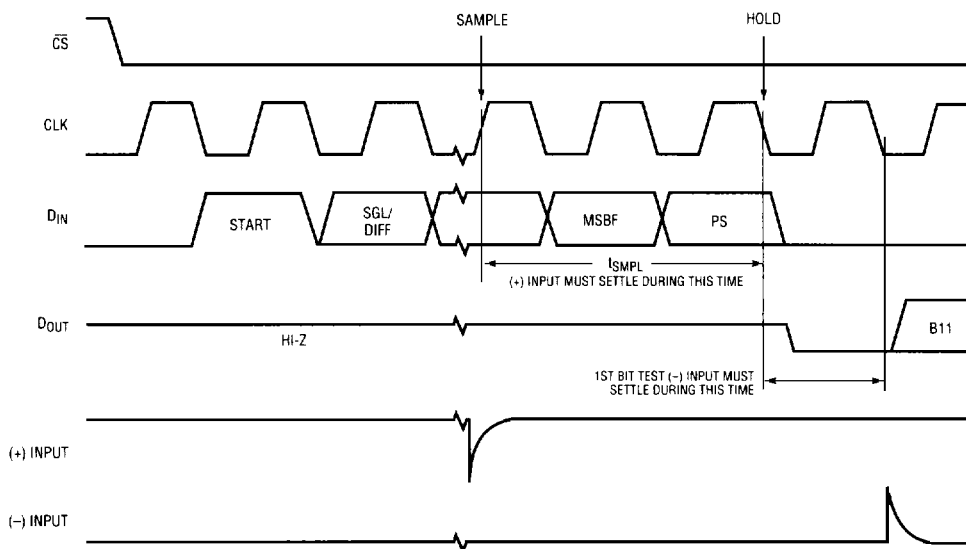
Figure 8. “+” and “-” Input Settling Windows
