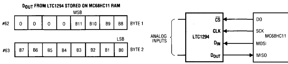
Hardware and Software Interface to Motorola MC68HC11
