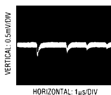
Figure 13. Adequate Reference Settling (LT1027)
