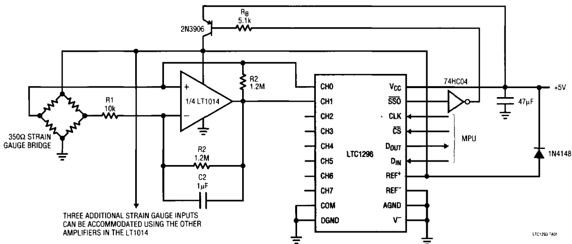
12-Bit Data Acquisition System with Power Shutdown
