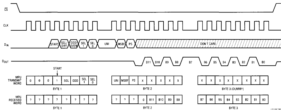
Data Exchange Between LTC1294 and MC68HC11
