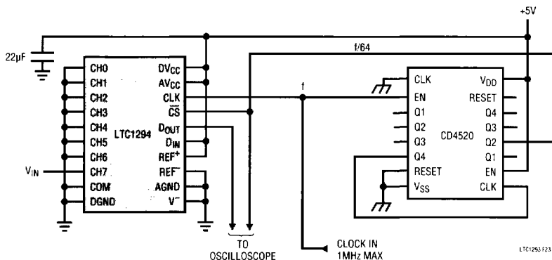
Figure 23. "Quick Look" Circuit for the LTC1294/6
