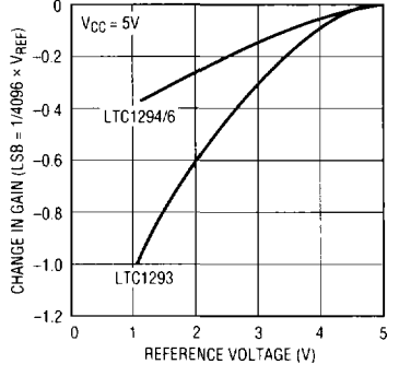
Change in Gain vs Reference Voltage
