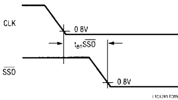
Voltage Waveform for t_{enSS0}
