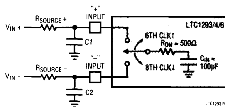
Figure 7. Analog Input Equivalent Circuit
