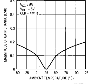
Change in Gain vs Temperature
