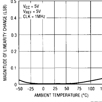
Change in Linearity vs Temperature
