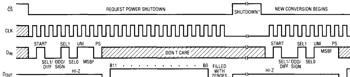
Power Shutdown Operating Sequence Example: Differential Inputs (CH4 + , CH5 - ), Unipolar Mode and MSB-First Data
