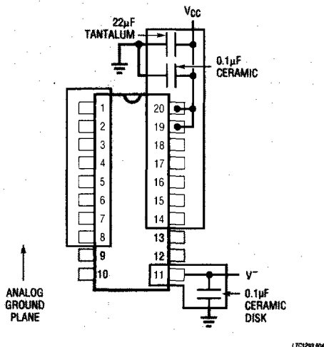
Figure 4. Ground Plane for the LTC1293/4/6
