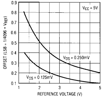
Unadjusted Offset Voltage vs Reference Voltage
