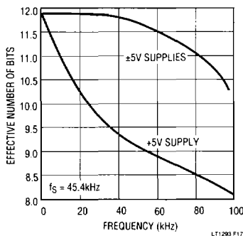
Figure 17. LTC1294 ENOB vs Input Frequency
