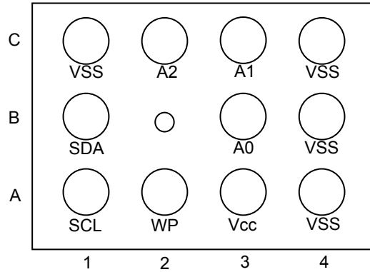
Fig.3 BU9897GUL-W(bottom view)
