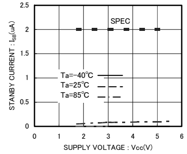
Fig.12 Standby operation I_{gb}
