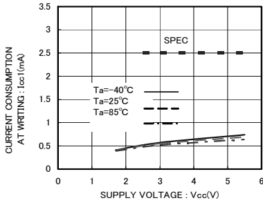
Fig.10 Current consumption at WRITE operation I_{cc1} (fsci=400kHz)
