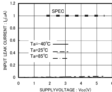
Fig.8 Input leak current I_{LI} (A0,A1,A2,SCL,WP)
