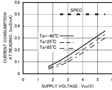
Fig.11 Current consumption at READ operation I_{cc2} (fsci=400kHz)
