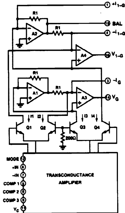
SSM-2018 FUNCTIONAL DIAGRAM
