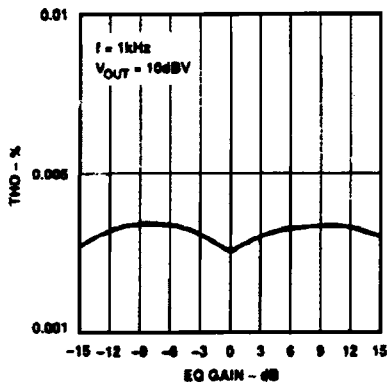
Figure 31. Equalizer THD+N vs. Gain
