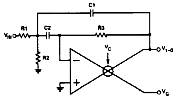
b. Voltage-Controlled Inverting Bandpass Filter
