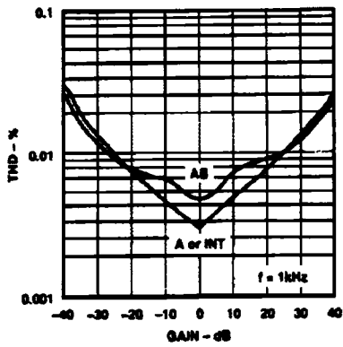
Figure 13. OVCE THD vs. Gain
