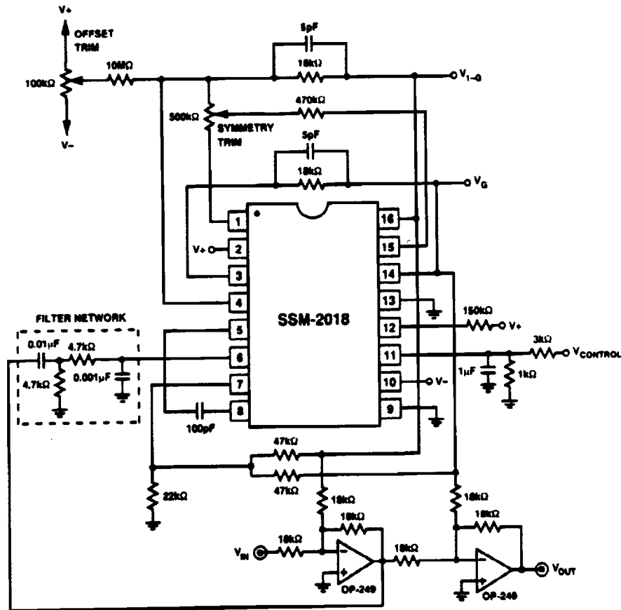
Figure 30. Voltage Controlled Equalizer Application Circuit
