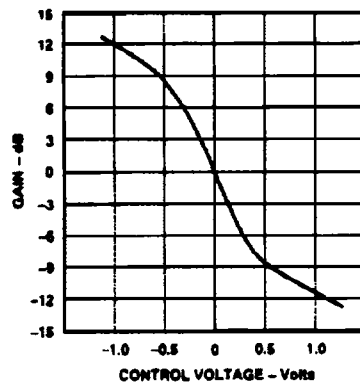
Figure 34. Equalizer Gain vs. Control Voltage
