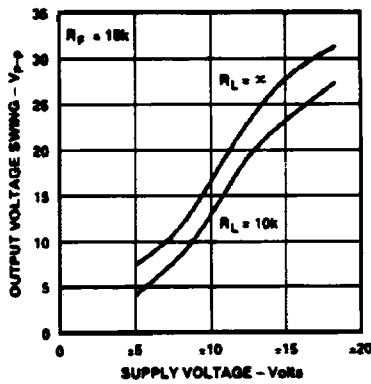
Figure 1. Maximum Output Swing vs. Supply Voltage
