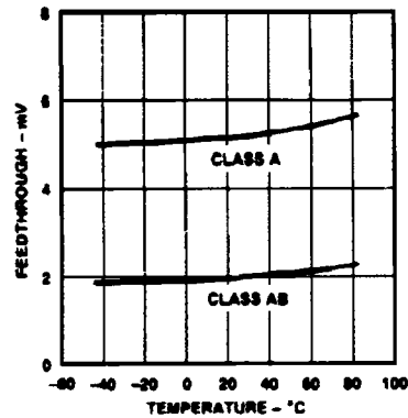
Figure 3. Trimmed Feedthrough vs. Temperature
