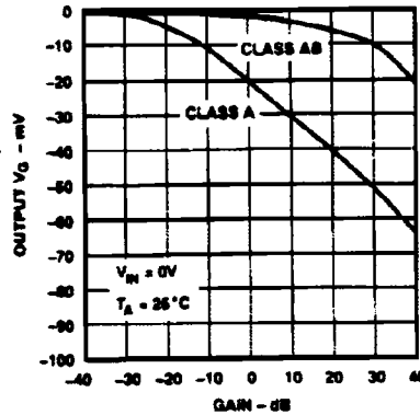
Figure 17. OVCE Output vs. Gain
