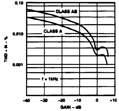
Figure 25. VCP THD+N vs. Gain
