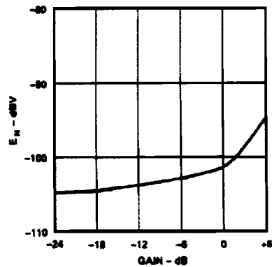
Figure 29. VCP Noise vs. Gain, Class AB Operation
