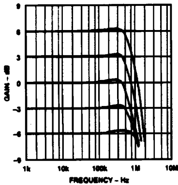
Figure 28. VCP Bandwidth vs. Gain, Class AB Operation
