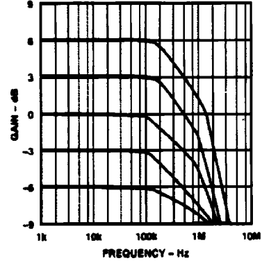
Figure 27. VCP Bandwidth vs. Gain, Class A Operation
