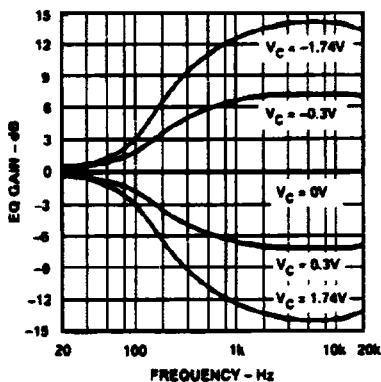
Figure 33. Equalizer Frequency Response vs. Gain
