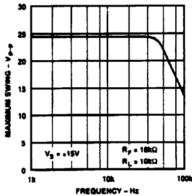
Figure 2. Maximum Output Swing vs. Frequency
