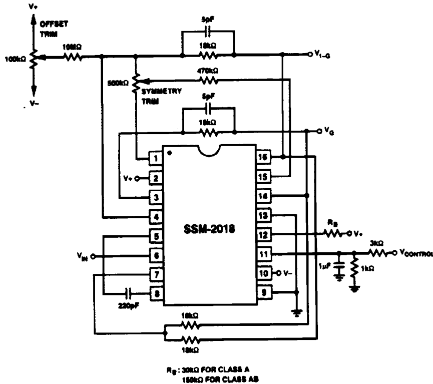
Figure 22. VCP Application Circuit
