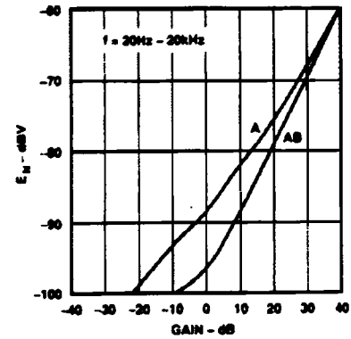
Figure 21. VCA/OVCE Noise vs. Gain
