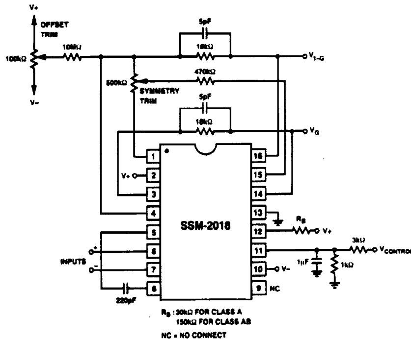
Figure 12. OVCE Application Circuit
