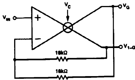
Figure 10. Basic VCP Connection
