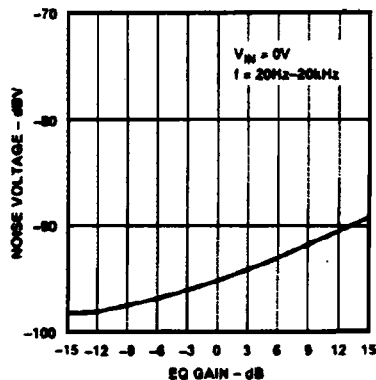
Figure 32. Equalizer Noise vs. Gain
