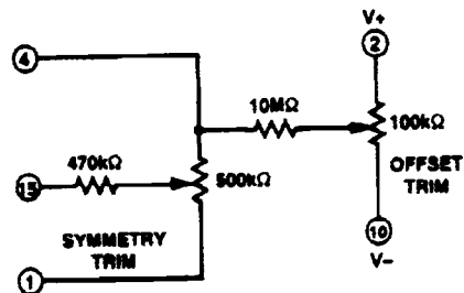
Figure 11. Symmetry and Offset Trim Network
