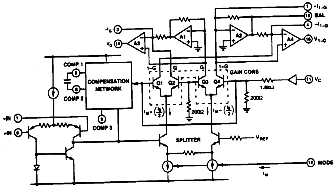
Figure 5. SSM-2018 Functional Diagram
