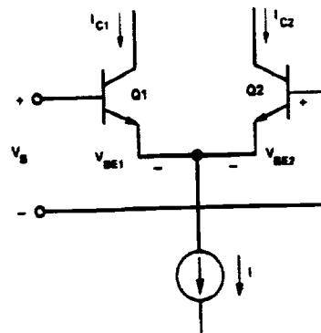
Figure 6. The OVCE Gain Core Differential Pair
