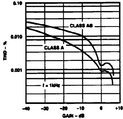
Figure 26. VCP THD vs. Gain
