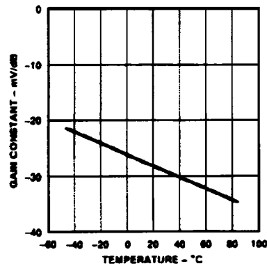
Figure 4. Gain Constant vs. Temperature
