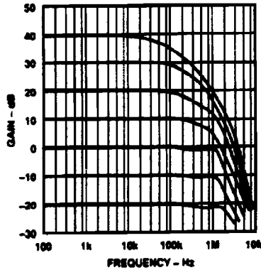
Figure 14. OVCE Bandwidth vs. Gain
