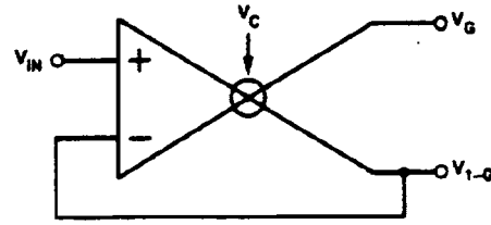
Figure 8. OVCE Follower/VCA Connection
