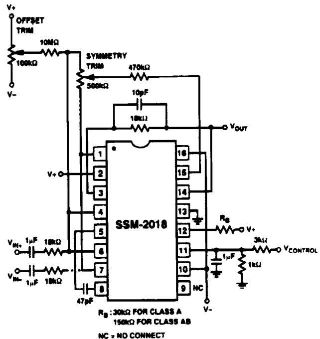
Figure 18. Simple VCA Application Circuit
