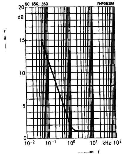
Noise figure F = f(f) I_C = 0.2\text{ mA}, R_s = 2\text{ k}\Omega, V_{CE} = 5\text{ V}
