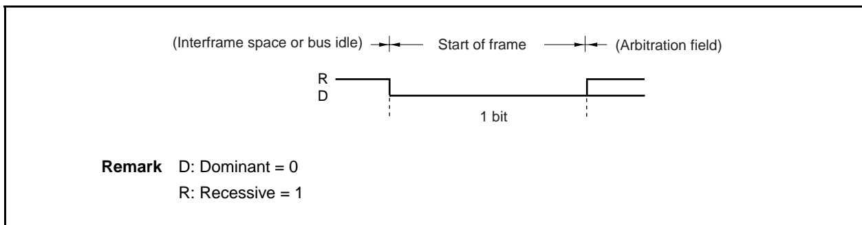
Figure 15-5. Start of Frame (SOF)
