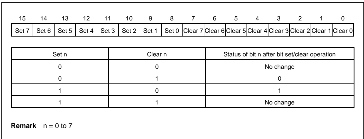
Figure 15-26. Bit Status After Bit Setting/Clearing Operations
