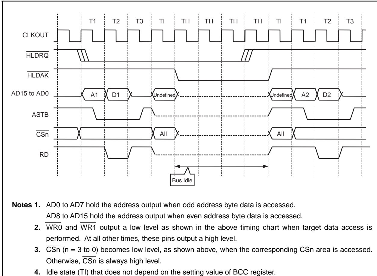
Figure 5-11. Basic Bus Cycle
