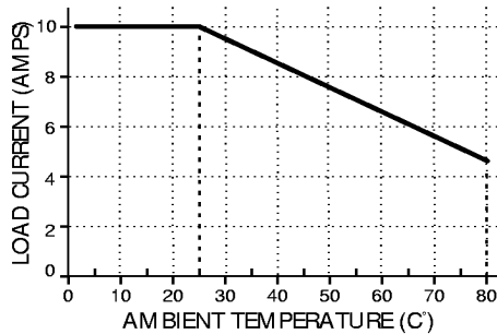
Fig.1 Convection Cooling
