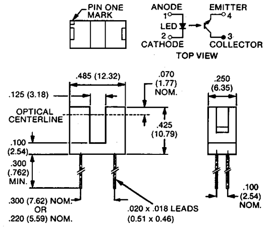
Package 7 Dimensions
