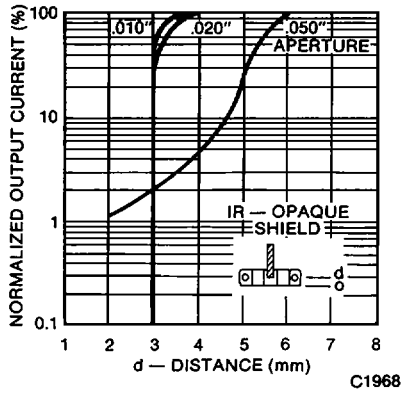
Fig. 7. Normalized Output Current vs. Lateral Shield Displacement
