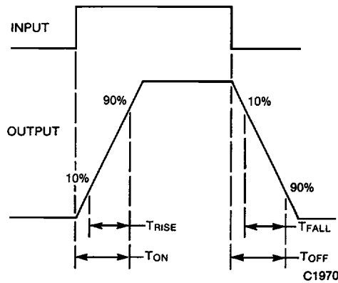
Fig. 9. Definition of Switching Parameters
