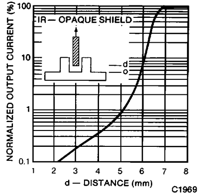
Fig. 8. Normalized Output Current vs. Vertical Shield Displacement
