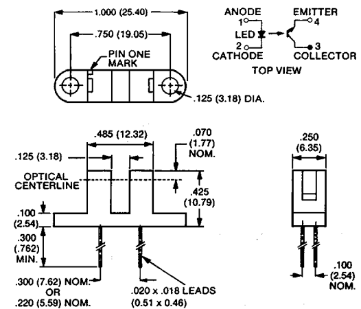
Package 6 Dimensions
