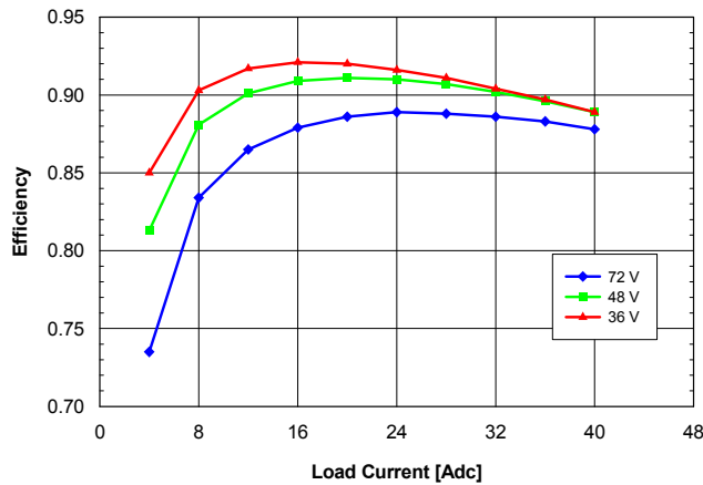
Fig. 2.5V.3: Efficiency vs. load current and input voltage for QME48T40025 converter mounted horizontally with air flowing from pin 1 to pin 3 at a rate of 300 LFM (1.5 m/s) and T_a = 25\text{ }^{\circ}\text{C} .
