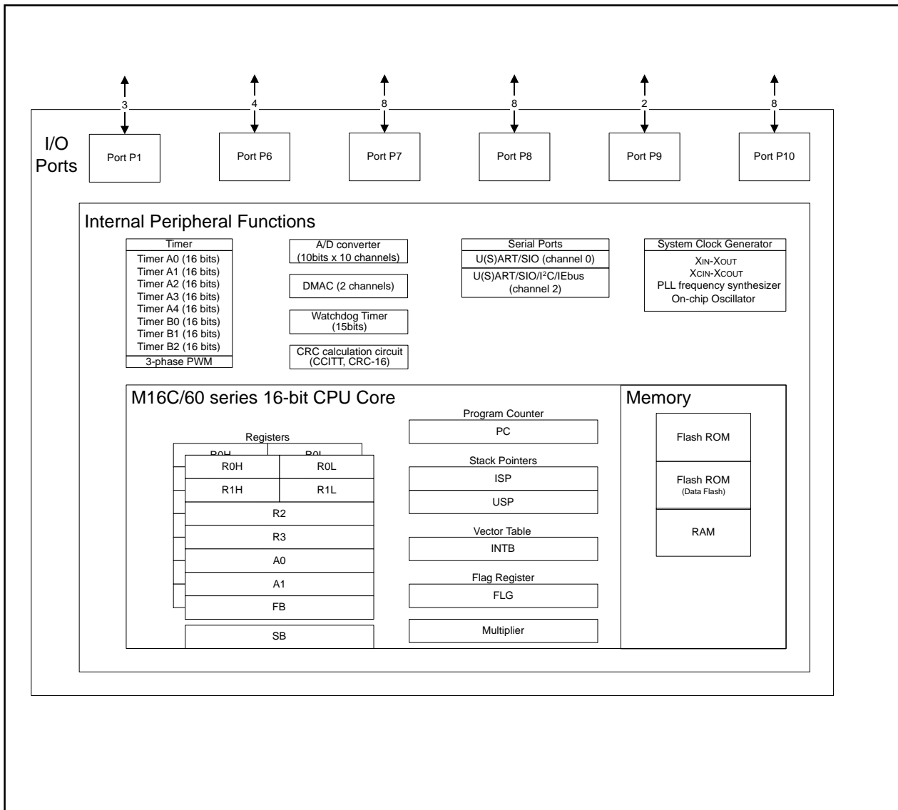
Figure 1.2. M16C/26A Group, 42-pin Block Diagram
