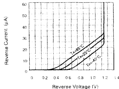
Reverse Characteristics
