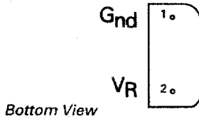
E-Line, 2 pin Package Suffix - Y
