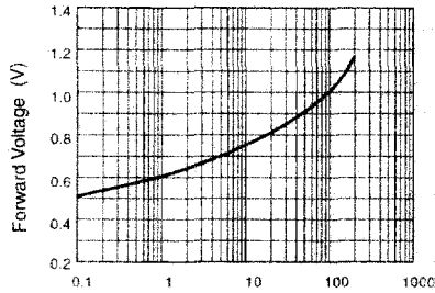
Forward Characteristics
