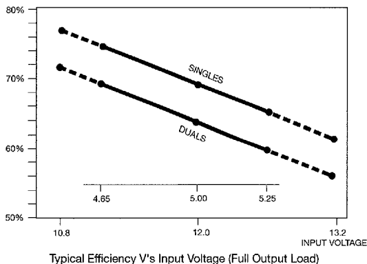
Typical Efficiency V's Input Voltage (Full Output Load)
