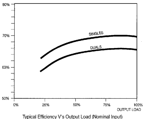
Typical Efficiency V's Output Load (Nominal Input)
