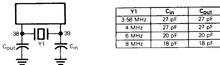
FIGURE 12 – CRYSTAL SPECIFICATIONS
