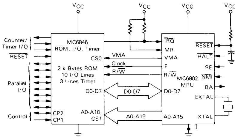
TYPICAL MICROCOMPUTER
