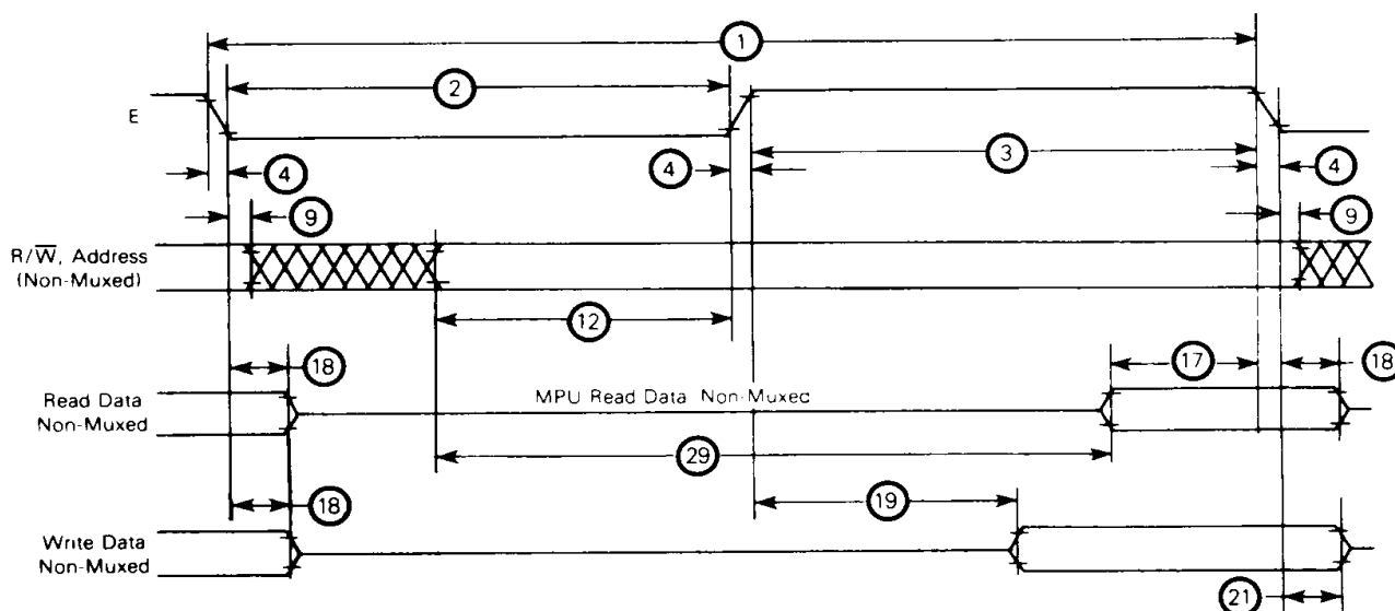
FIGURE 2 — BUS TIMING
