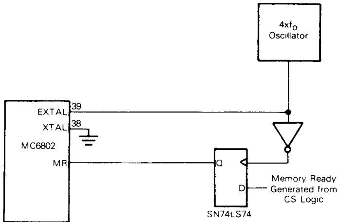
FIGURE 14 — MEMORY READY SYNCHRONIZATION
