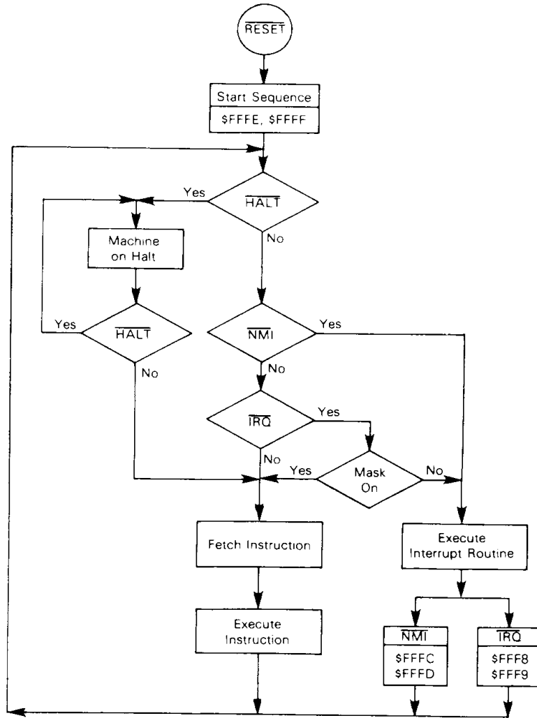
FIGURE 11 — MPU FLOWCHART
