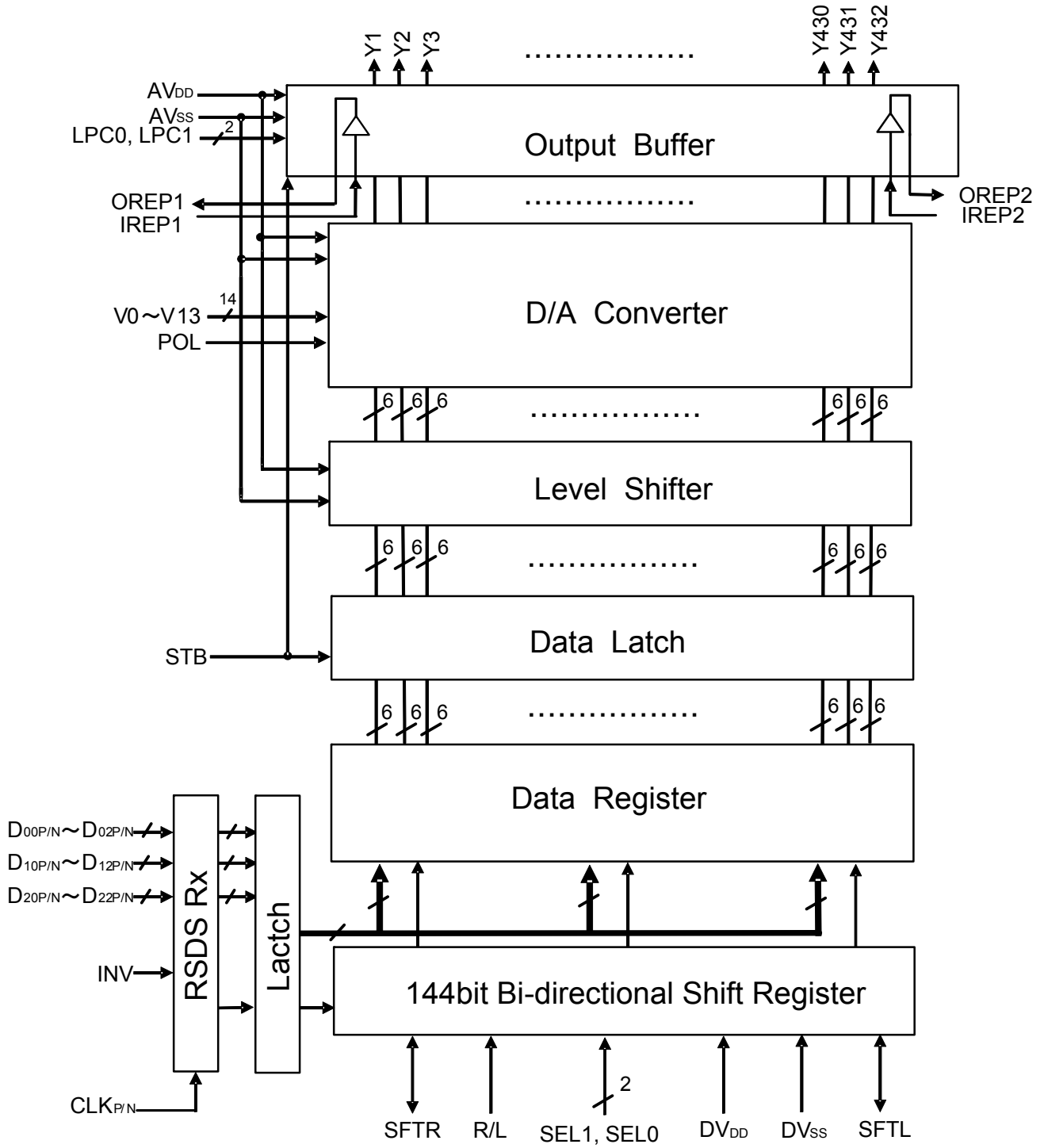
Fig.1 Block diagram
