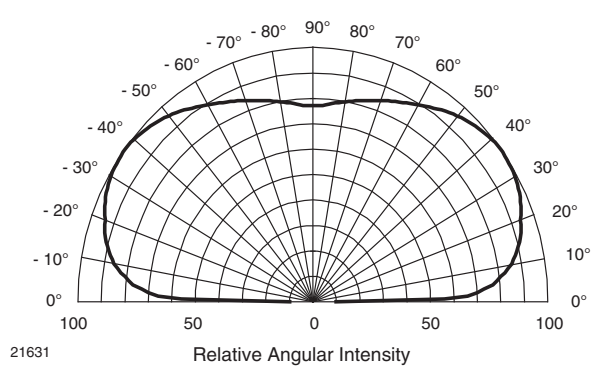
Fig. 2 - Radiant Characteristics I_{\text{rel}} = f(\varphi)
