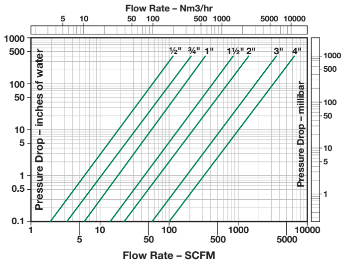
Pressure Drop
