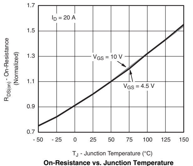
I_D = 20\text{ A} V_{GS} = 10\text{ V} V_{GS} = 4.5\text{ V} On-Resistance vs. Junction Temperature
