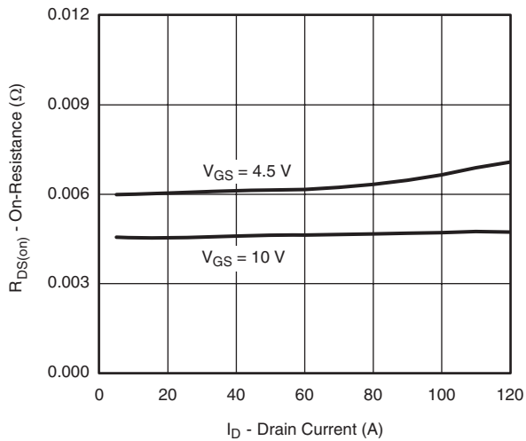
V_{GS} = 4.5\text{ V} V_{GS} = 10\text{ V} On-Resistance vs. Drain Current and Gate Voltage
