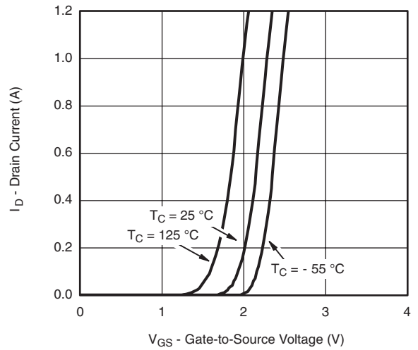
T_C = 25\text{ °C} T_C = 125\text{ °C} T_C = -55\text{ °C} Transfer Characteristics
