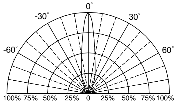
Fig.6 Directive Radiation
