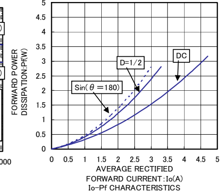
Io-Pf CHARACTERISTICS
