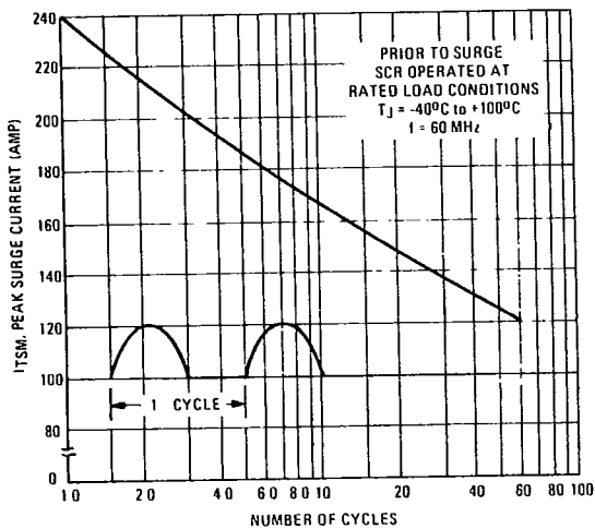
FIGURE 3 - 60 Hz SURGES
