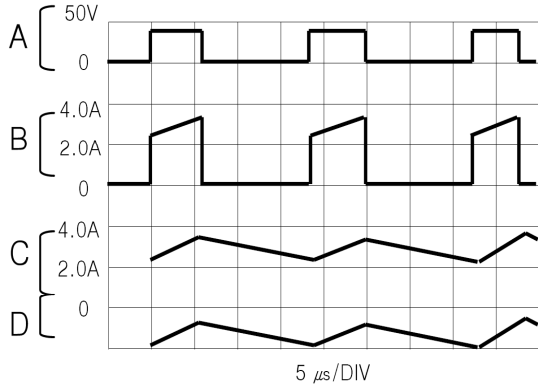
Figure 13. Switching Waveforms
