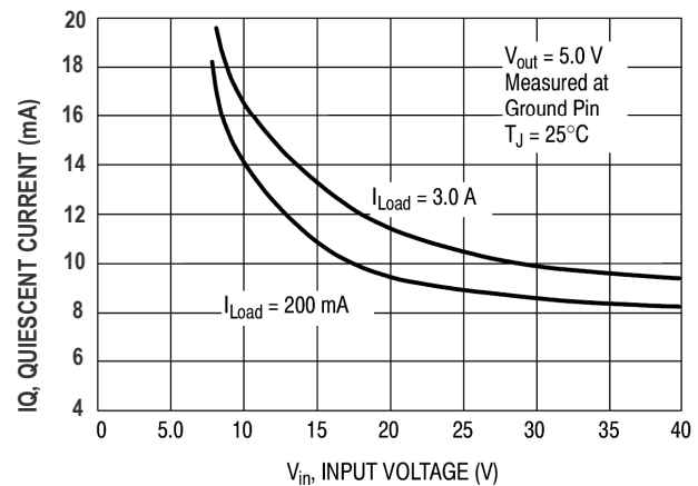
Figure 6. Quiescent Current
