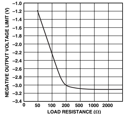
TPC 9. Typical Output Voltage Swing vs. Load Resistance (Negative Output Swing Limits First)
