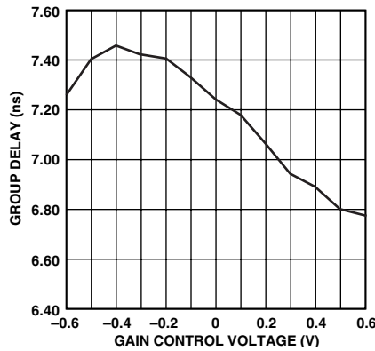
TPC 5. Group Delay vs. Gain Control Voltage
