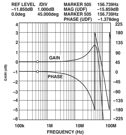
TPC 3. Frequency and Phase Response vs. Gain (Gain = +10 dB, P_{IN} = -30 dBm, Pin 5 Connected to Pin 7)
