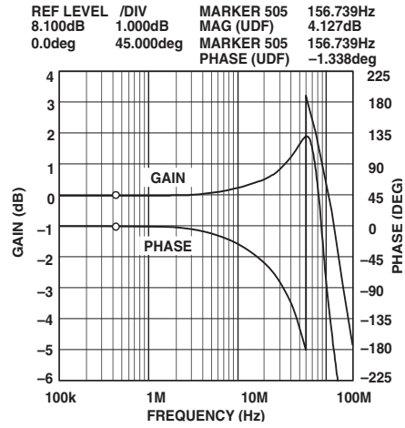
TPC 2. Frequency and Phase Response vs. Gain (Gain = -10 dB, P_{IN} = -30 dBm, Pin 5 Connected to Pin 7)
