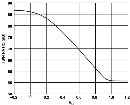
Figure 14. IS/N RATIO vs. Control Voltage—Low Ripple Mode
