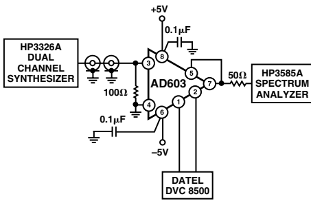
TPC 19. Test Setup Used for: Noise Figure, Third Order Intercept and 1 dB Compression Point Measurements
