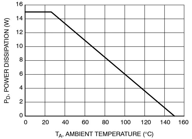
Figure 8. Power Derating
